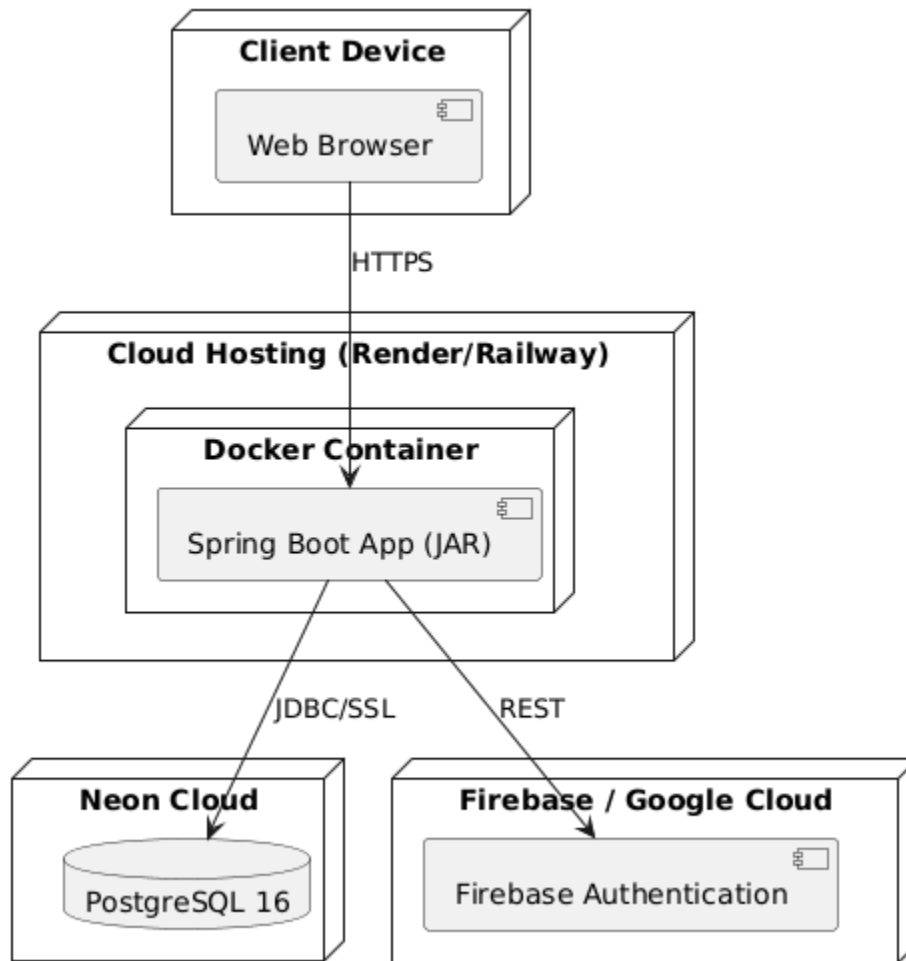
Deployment Diagram
